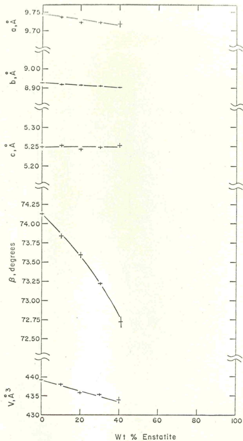
Fig. 5. Unit-cell parameters along the join diopside-enstatite.
